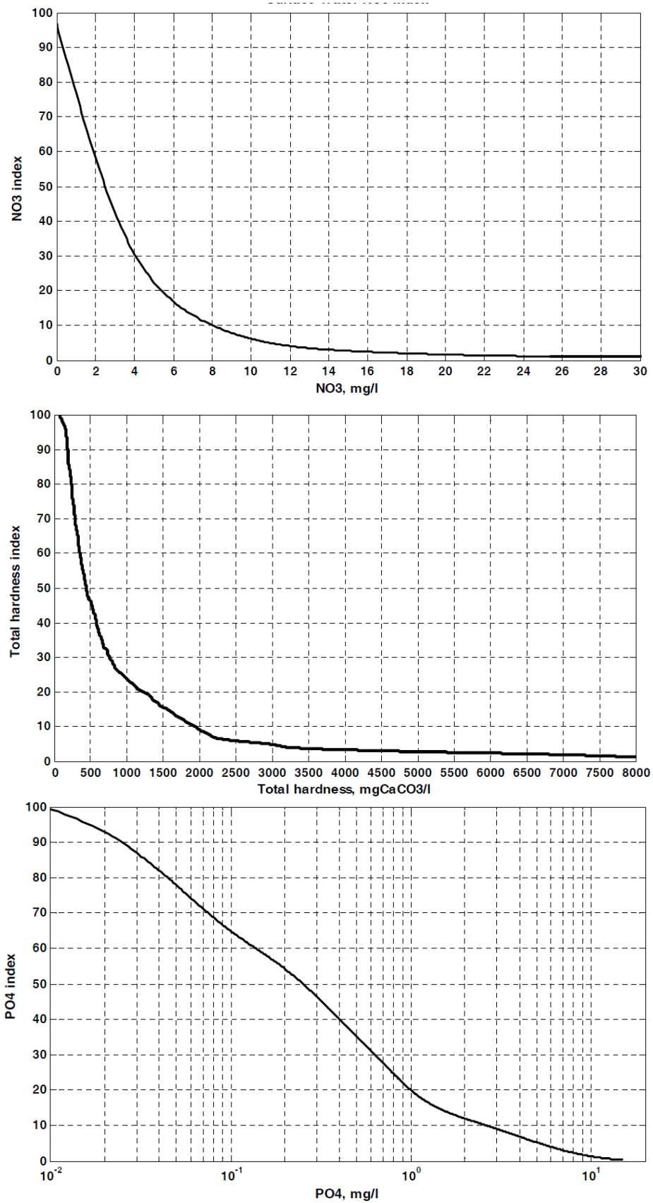
Fig. 2. Standard curves to calculate the sub-index of nitrate, total hardness and phosphate
