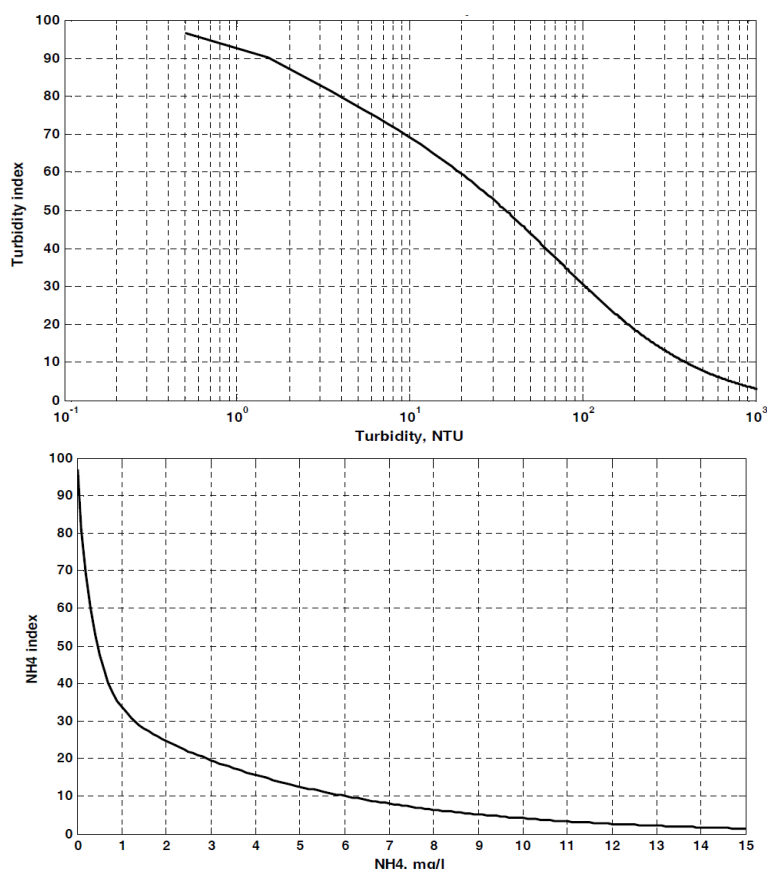
Fig. 4. Standard curves to calculate the sub-index of turbidity and ammonium
