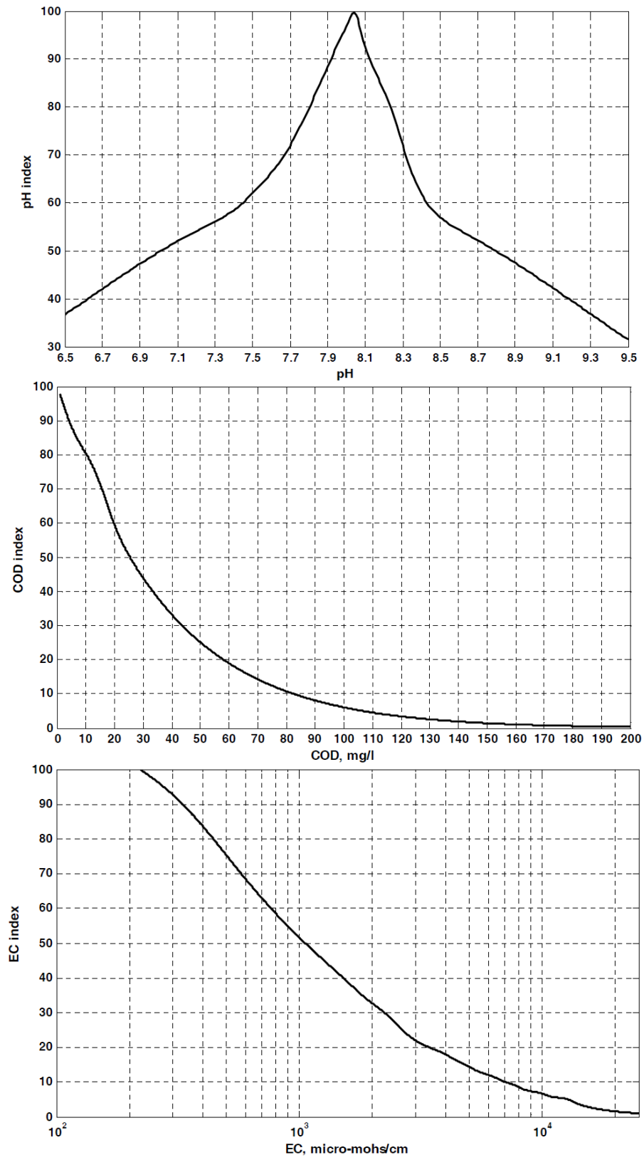
Fig. 3. Standard curves to calculate the sub-index of pH, COD and EC
