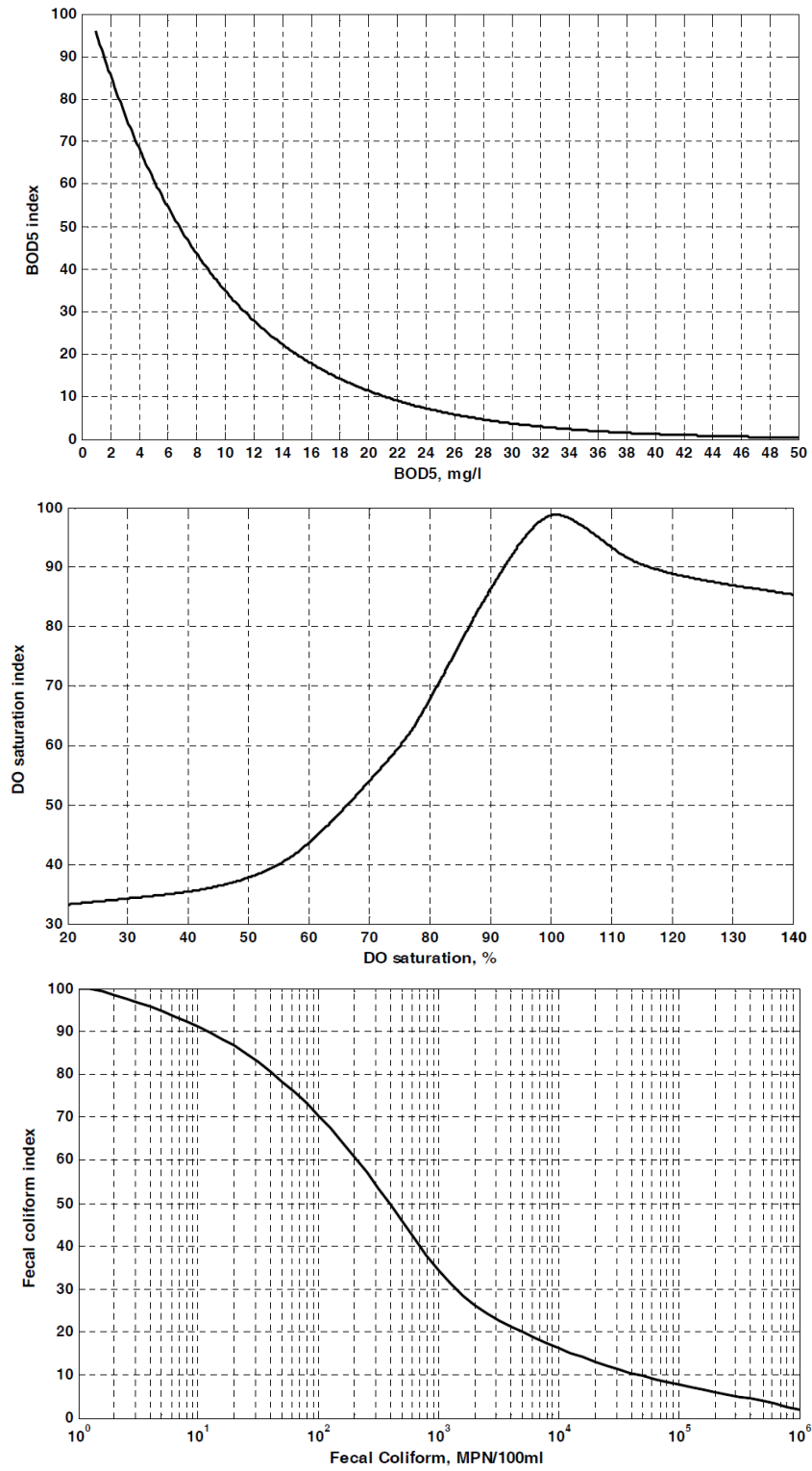
Fig. 1. Standard curves to calculate the sub-index of BOD 5 , dissolved oxygen and fecal coliform
