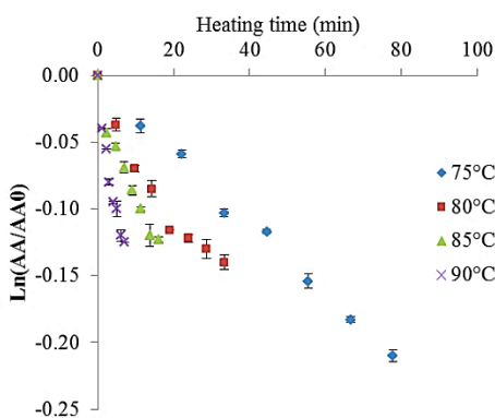
Fig. 2. Inactivation kinetic of Ascorbic acid during thermal processing of quince puree at 75 to 90°C.
