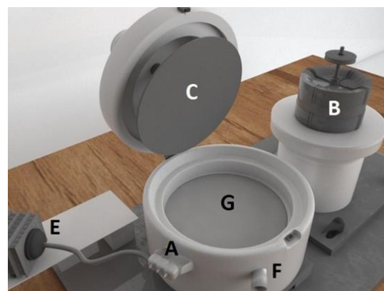
Fig. 1. Dry-based extractor designed for separation of the mucilage from the mucilaginous seeds: (A) Feed inlet, (B) Rotor, (C) Mobile abrasion surface, (E) Air compressor, (F) Outlet, (G) Stationary abrasion surface.
